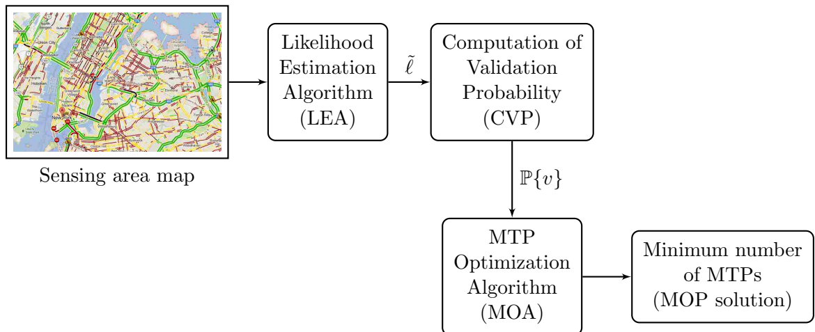
Figure 3.3. Block scheme of the proposed FIRST framework.
